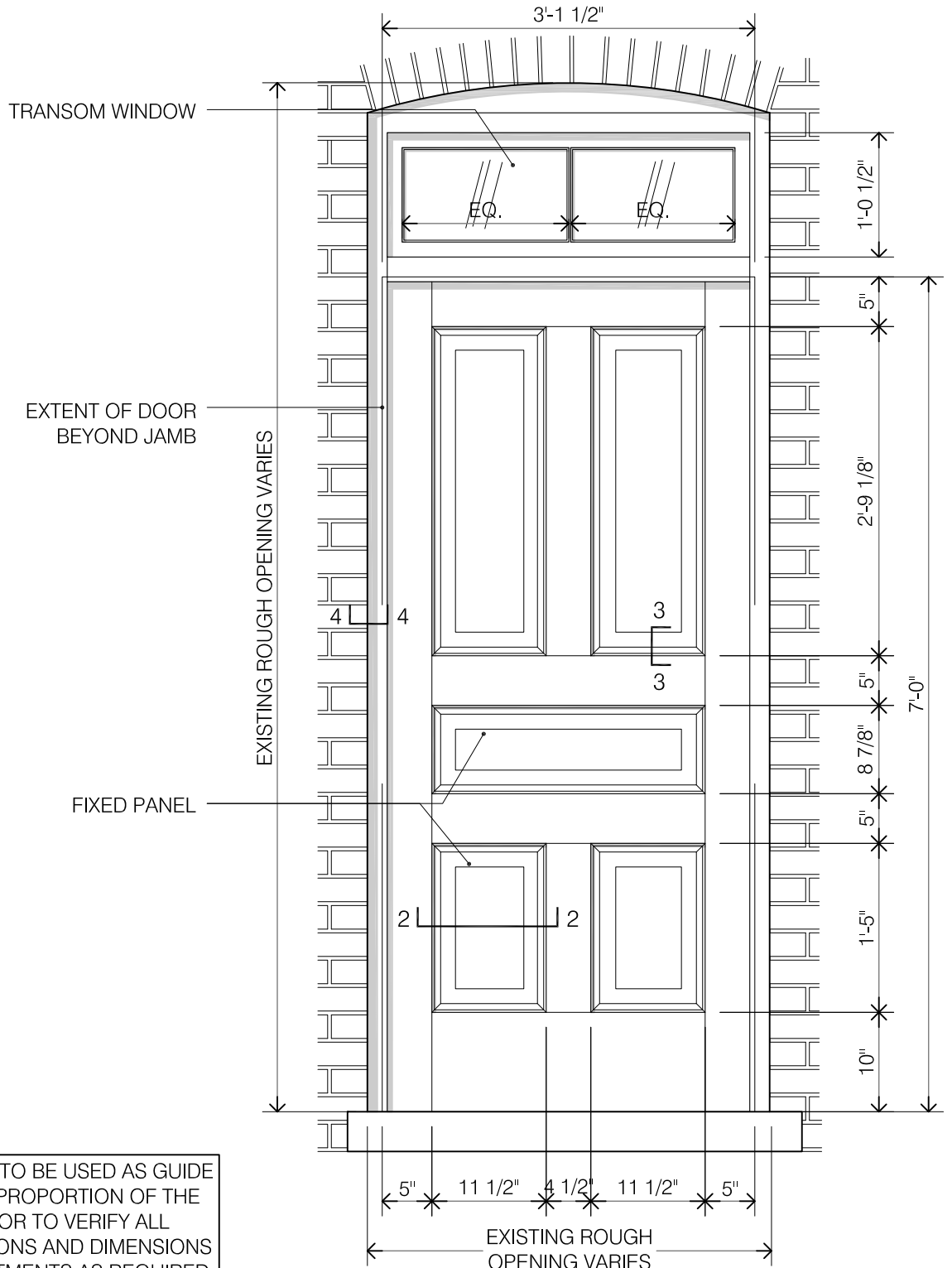
1 EXTERIOR DOOR ELEVATION SCALE: 3/4" = 1'-0"
