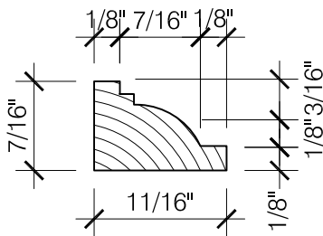
5 PANEL STOP DETAIL SCALE: 1'-0" = 1'-0"
