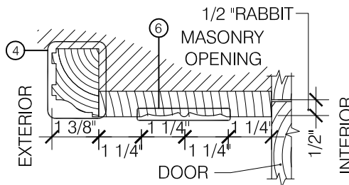
3 SECTION AT BRICK MOLD AND JAMB SCALE: 3" = 1'-0"
