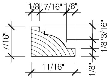
6 PANEL STOP DETAIL SCALE: 1'-0" = 1'-0"
