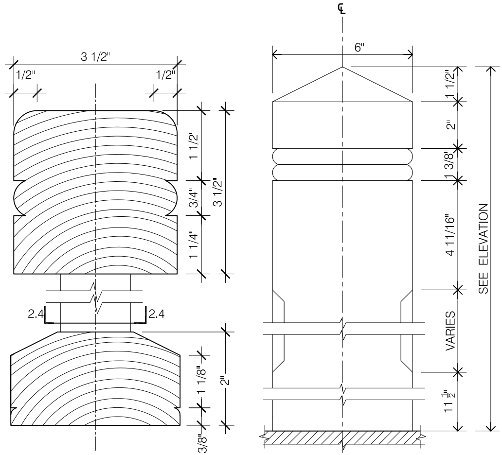
2.3 SECTION AT HAND RAIL SCALE: 3" = 1'-0"
