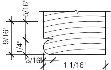
4 TYP. DETAIL OF SCROLL WORK AT BRICK MOLD SCALE: 1'-0" = 1'-0"
