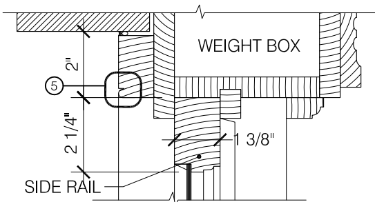
2 SECTION AT JAMB SCALE: 3" = 1'-0"
