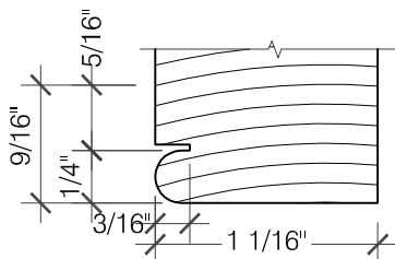
5 TYP. DETAIL OF SCROLL WORK AT BRICK MOLD SCALE: 1" = 1'-0"
