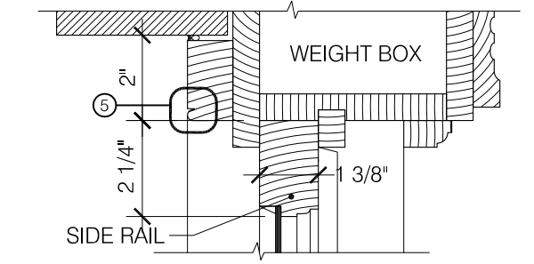
2 SECTION AT JAMB SCALE: 3" = 1'-0"
