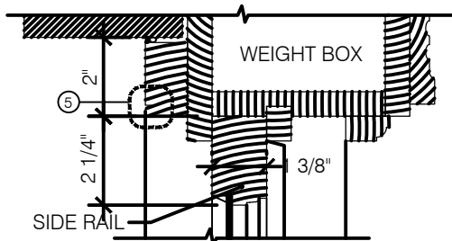
2 SECTION AT JAMB SCALE: 3" = 1'-0"
