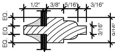
4 TYPICAL MUNTIN DETAIL SCALE: 1'-0" = 1'-0"
